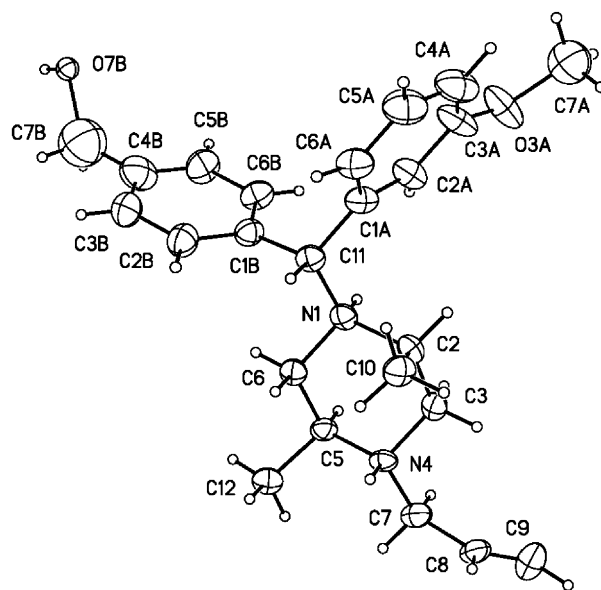
Figure 1. Displacement ellipsoid plot of (+)-4-[(α R )-α-(4-allyl-(2 S ,5 S )-dimethyl-1-piperazinyl)-(3-methoxyphenyl)methyl]-benzyl alcohol dihydrobromide ( 10 ·2HBr) drawn at 30% probability level. The bromine ions have been omitted for clarity.
