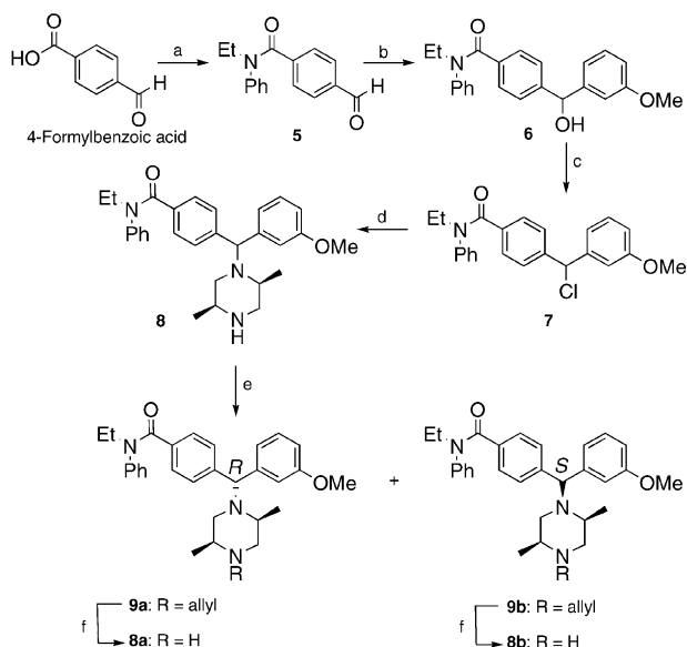
Scheme 1. Conditions: (a) N -ethylaniline, EDCI, 10 °C to rt, CH 2 Cl 2 , 88%; (b) 3-MeO-PhMgBr, 10 °C to rt, THF, 78%; (c) HCl, CHCl 3 , rt, 97%; (d) (2 S ,5 S )-dimethylpiperazine, NaHCO 3 , CH 3 CN, reflux, 72%; (e) allyl bromide, NaHCO 3 , DMF, 80 °C, 95%; (f) 10% Pd/C, cat CH 3 CO 2 H, H 2 O, reflux.
