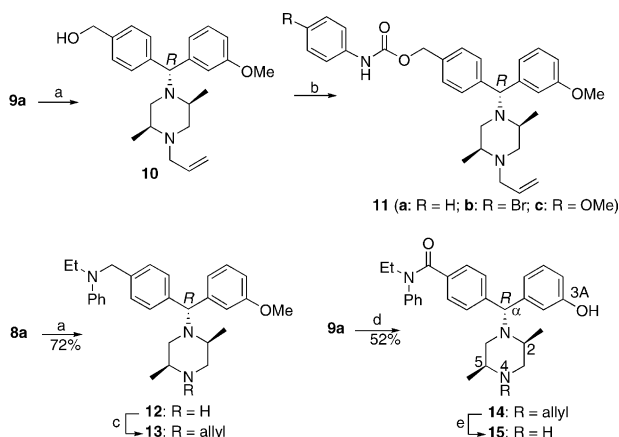
Scheme 2. Conditions: (a) LiAlH 4 , Et 2 O, reflux; (b) arylisocyanate, C 6 H 6 , rt, 89–94%; (c) allyl bromide, NaHCO 3 , DMF, 80 °C, 97%; (d) BBr 3 Me 2 S in CH 2 Cl 2 , 1,2-dichloroethane, 60 °C, 52%; (e) 10% Pd-C, cat CH 3 CO 2 H, H 2 O, reflux, 73%.
